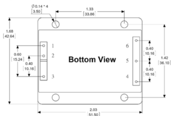
(Metal case shell with Heat-Sink)
